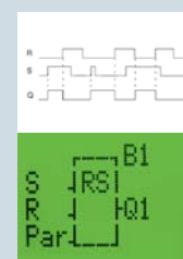
Latching relay
