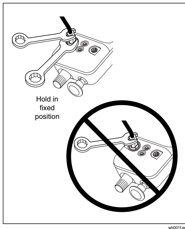
Figure 1. Connection Technique
