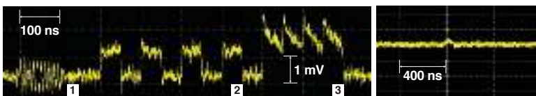
Earlier model Output rate of 1 V/A precludes observation of accurate waveforms as they are obscured by noise.
