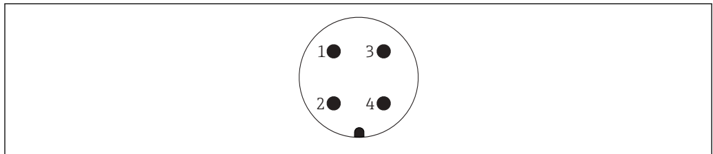
20 Pin assignment of 7/8" plug
