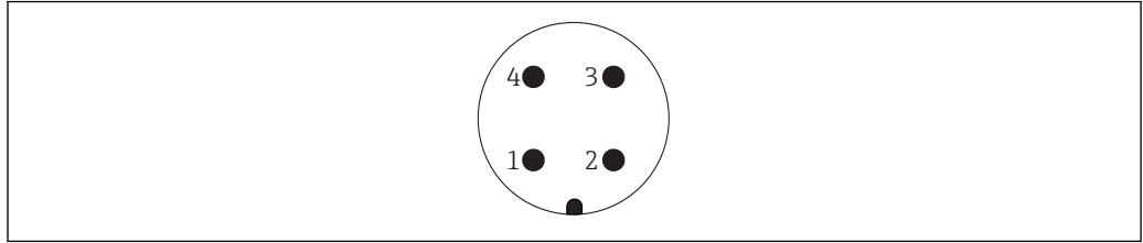
19 Pin assignment of M12 plug
