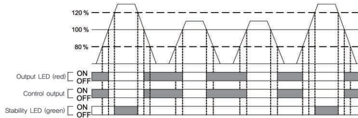
D.ON operation
