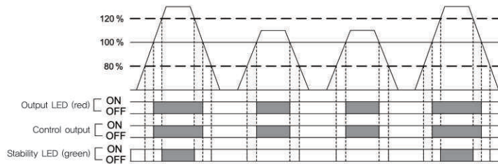
L.ON operation
