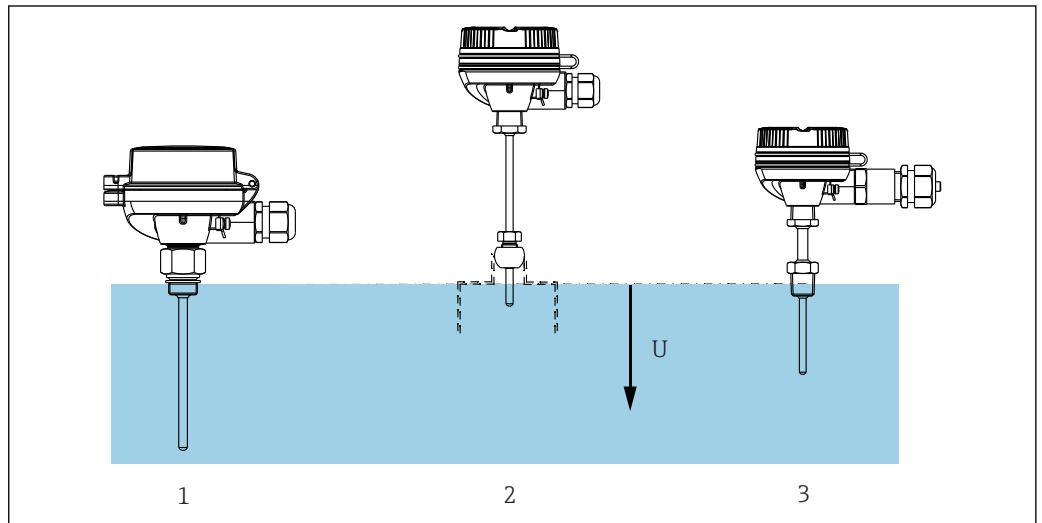
2 The thermometer is designed for direct process installation or in a locally installed thermowell
